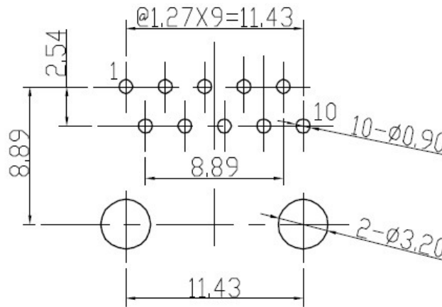
PC BOARD LAYOUT THICKNESS=1.60MM
